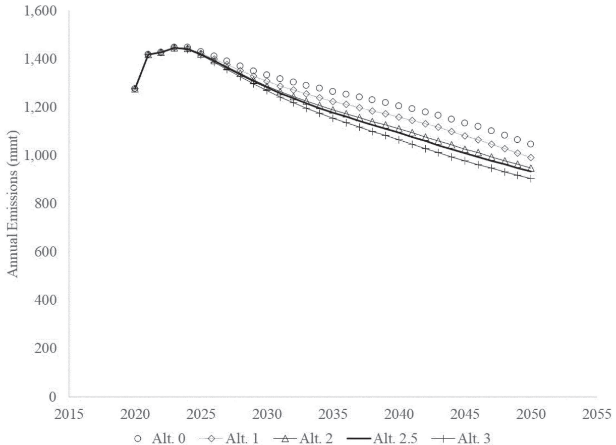
Figure II-5 – Estimated Annual CO 2 Emissions Attributable to Light-Duty On-Road Fleet
