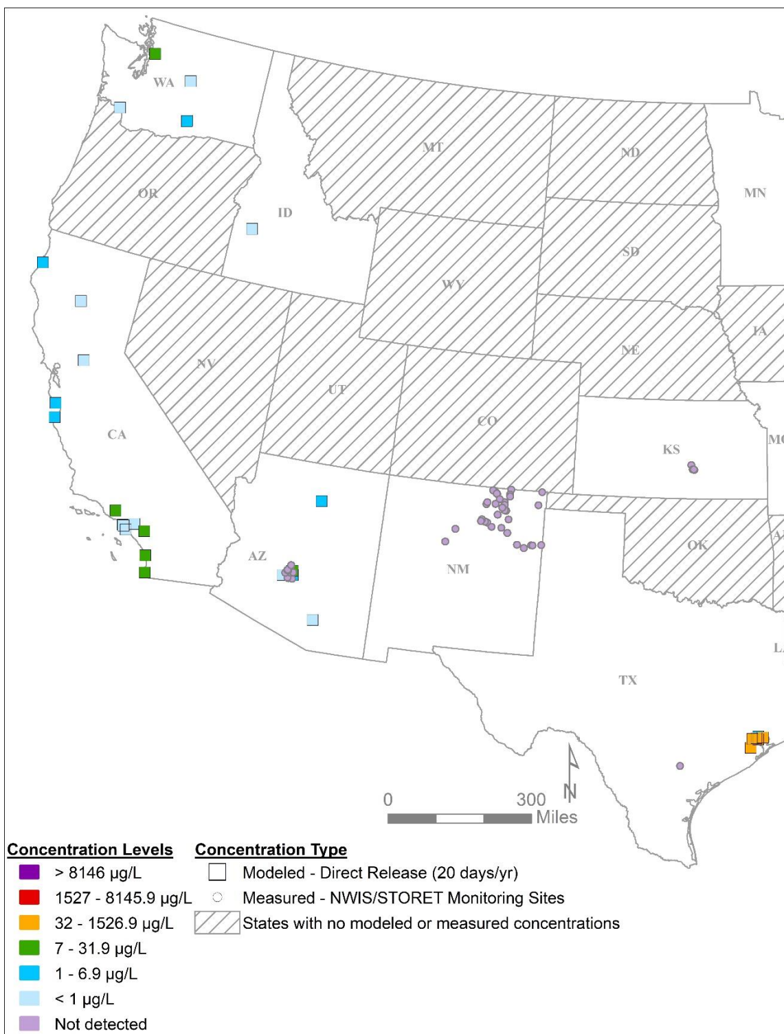
Figure 2-5. Concentrations of Methylene Chloride from Releasing Facilities (20 Days of Release Scenario) and Water Quality Exchange (WQX) Monitoring Stations: Year 2016, West U.S.
