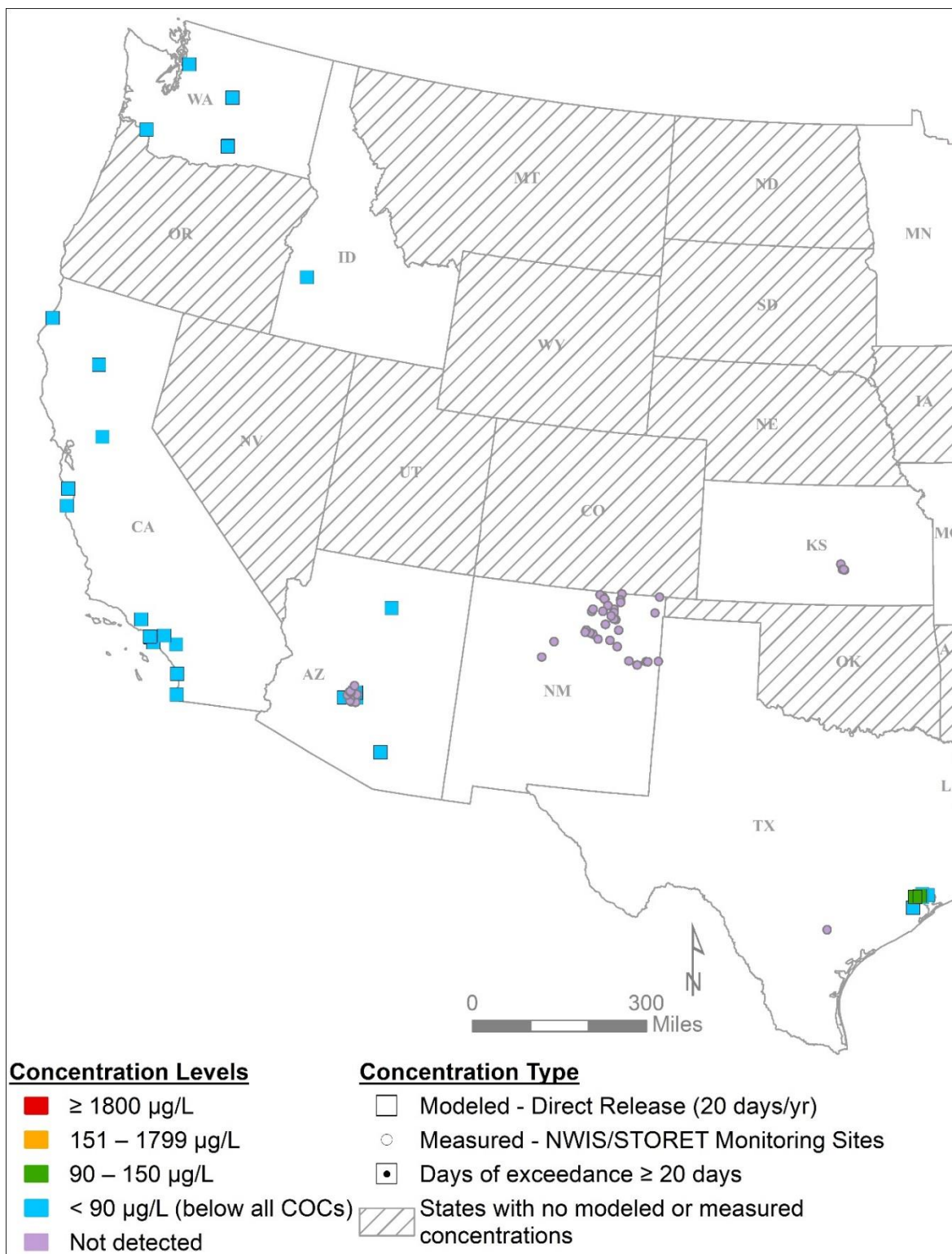
Figure 4-4. Concentrations of Methylene Chloride from Methylene Chloride-Releasing Facilities (20 Days of Release Scenario) and WQX Monitoring Stations: Year 2016, West U.S.
