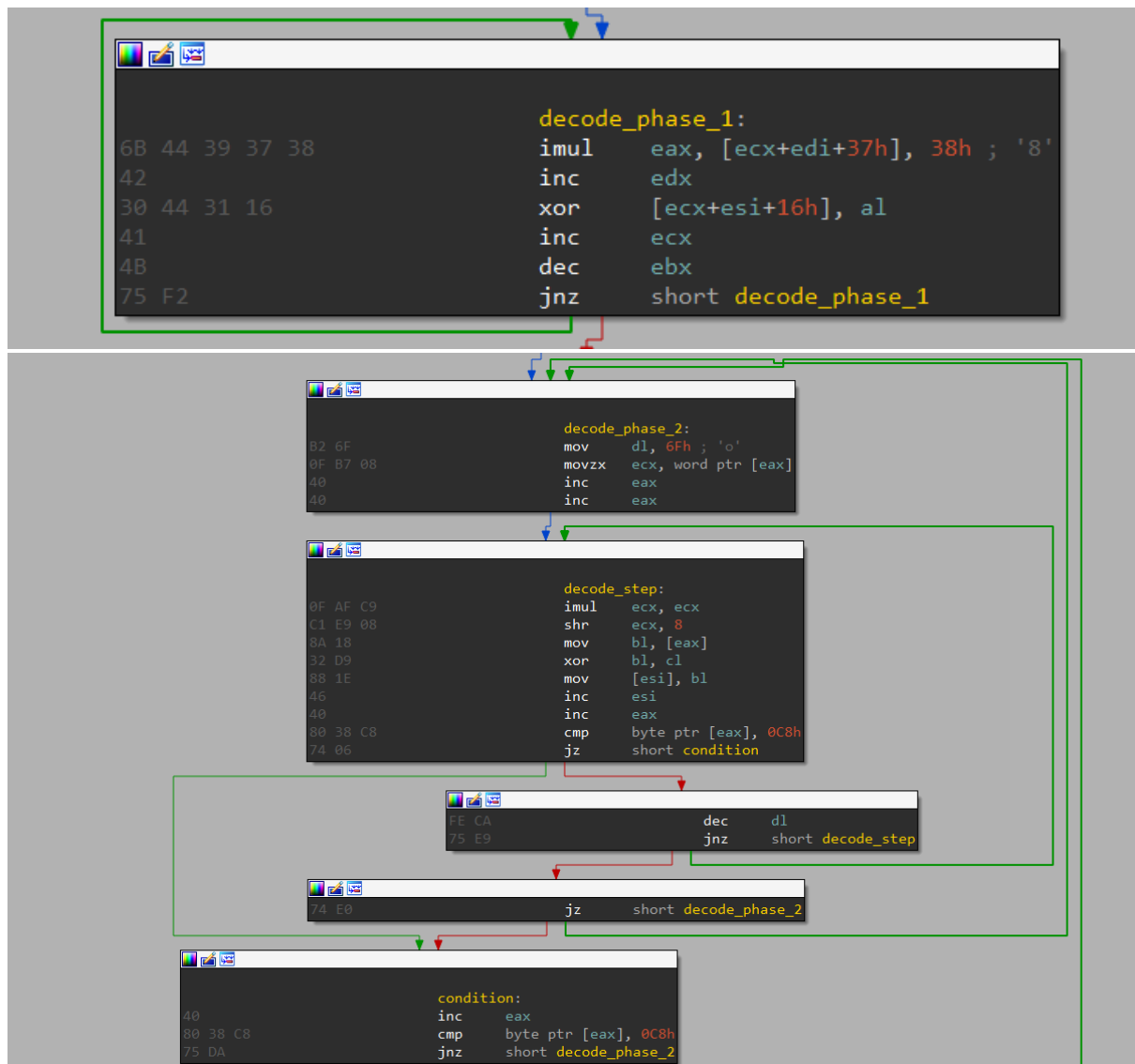
Figure: First and second phase of decoding the loader's payload.
