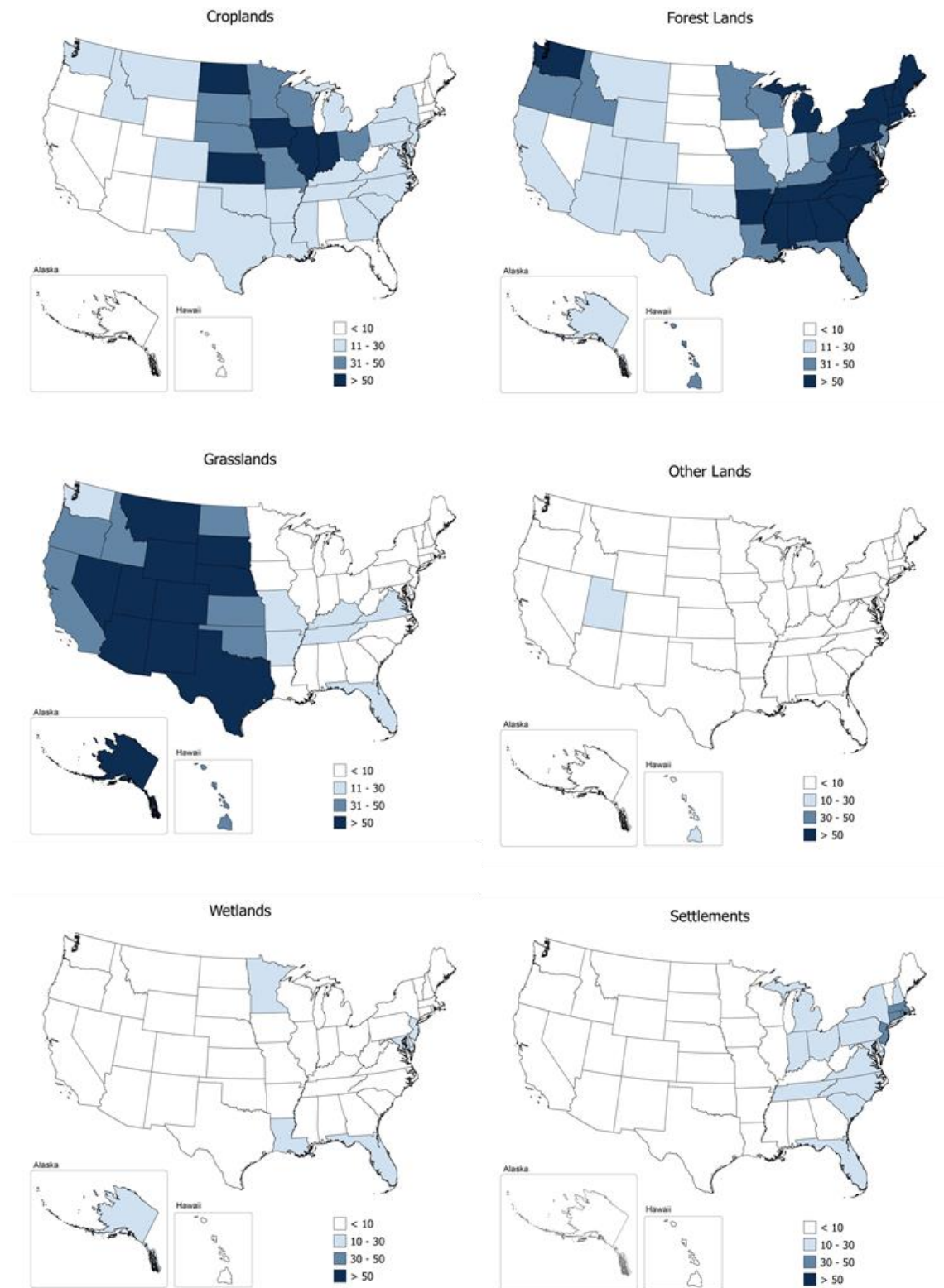
Figure 6-2: Percent of Total Land Area for Each State in the General Land-Use Categories for 2017
