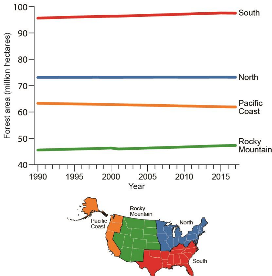
Figure 6-3: Changes in Forest Area by Region for Forest Land Remaining Forest Land in the conterminous United States and Alaska (1990-2017, Million Hectares)
