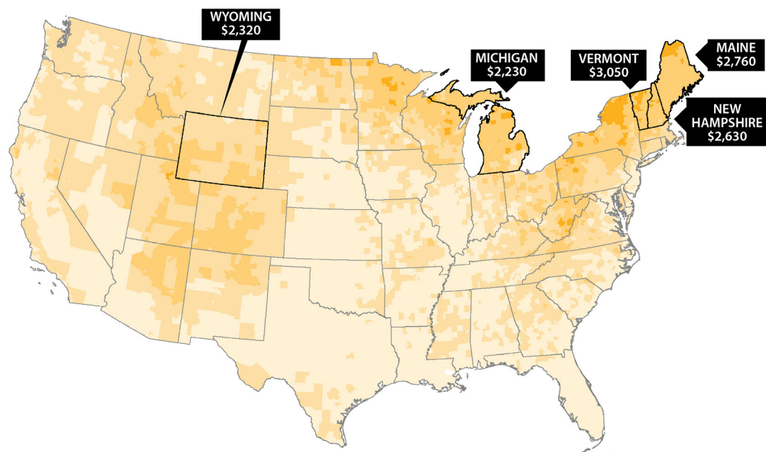
4°C of Global Warming
